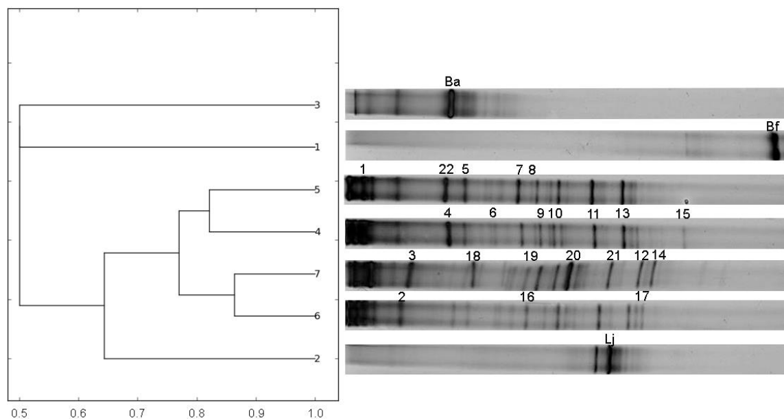
Figure 2. PCR-DGGE-profiles and dendrogram constructed from amplicons from the V3 region of 16S rRNA gene. PCR products were obtained from genomic DNA of the following probiotic bacteria; B. animalis lactis (lane 1); L. johnsonii strain C4 (lane 2); Bacillus sp strain B2 (lane 3). Lanes 4-7 showed similar amplicons but obtained from metagenomic DNA from fecal samples of Shortfin Silverside fed as follows: lane 4 -control group ( A. franciscana without probiotic bacteria); lane 5 - A. franciscana bio-encapsulating B. animalis subsp. lactis strain BB-12; lane 6 - A. franciscana bio-encapsulating L. johnsonii C4; lane 7 - A. franciscana bio-encapsulating Bacillus sp B2. Black numbers indicate DGGE bands that were excised and sequenced, microbial affiliations of those DGGE bands are summarized in Table 2. The bar numbers indicate the Euclidean distances.
